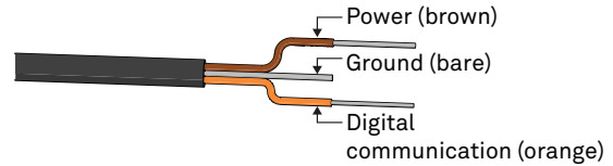
Figure 3 Pigtail cable
