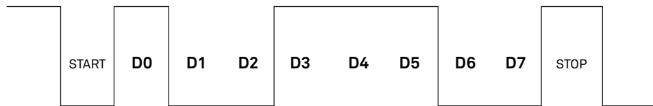
Figure 9 Example DDI serial transmission of the character 9 (0x39)
