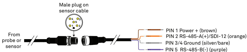
Figure 5 Four-wire M12 connector and pigtail adapter for use with screw terminals
