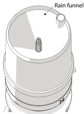
Figure 22 Rain funnel and pyranometer
