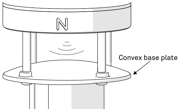
Figure 10 Anemometer
