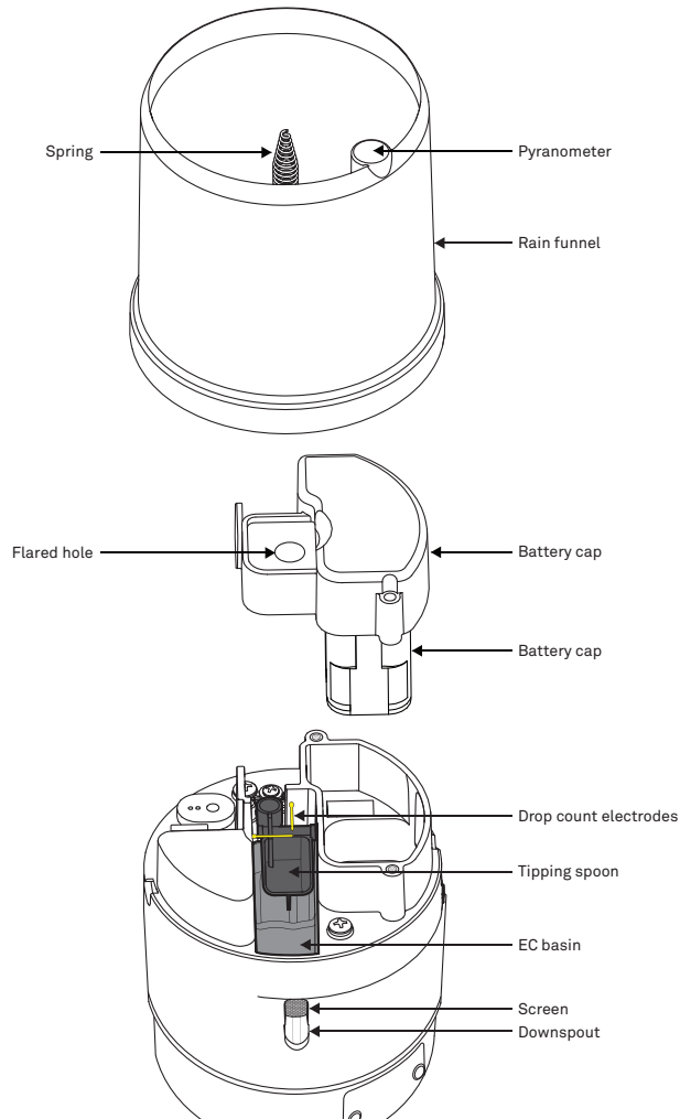
Figure 12 Rain funnel and rain gauge
