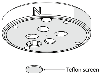
Figure 21 Teflon screen
